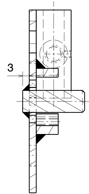
Section view J-J Scale: 1:1
